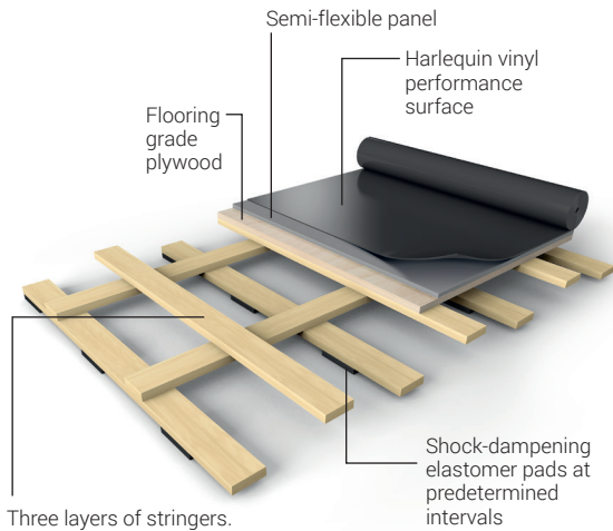
Three layers of stringers. Custom constructions possible with more layers for added shock absorption.
