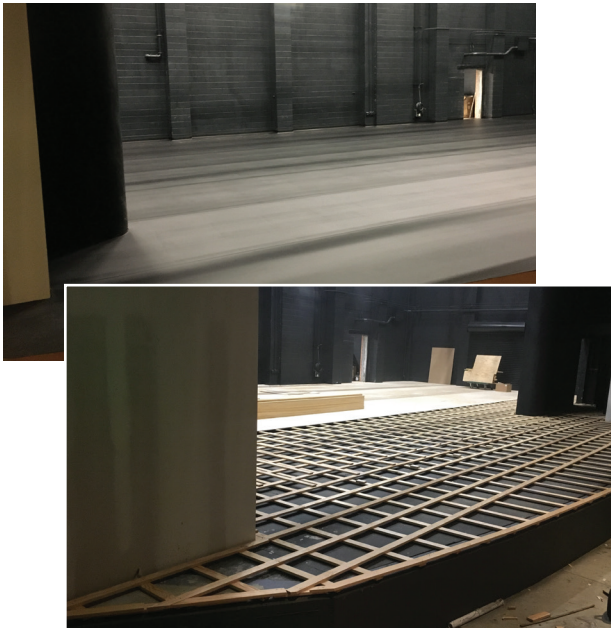
Kennesaw State University stage floor project featuring Harlequin WoodSpring and Harlequin Cascade.
